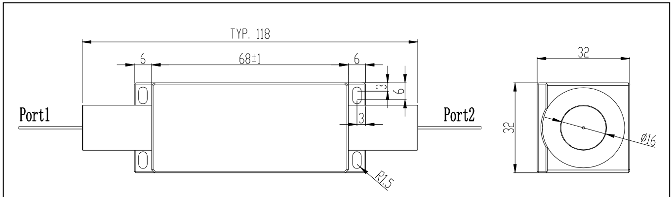
(Package dimensions in mm)
